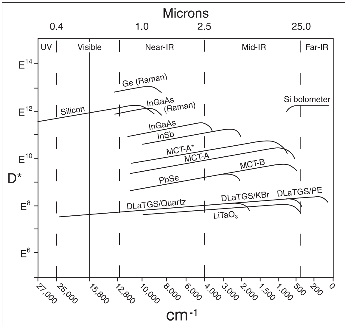
Figure 2: Graphical representation of detector D^* versus spectral range for Nicolet FT-IR detectors. The vertical line at 15798 cm^{-1} represents the helium neon (HeNe) laser emission band which is utilized for internal registration of spectral data.
