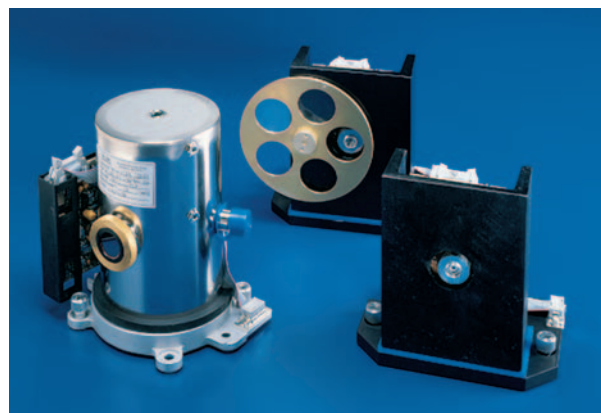
Figure 1: Vibrational spectroscopy detectors use a pre-aligned, pinned-in-place design and may be repositioned to other system locations with automatic recognition
